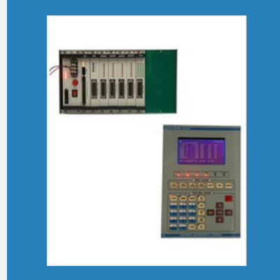
Programmable Logic Controller (PLC HP-02A)
