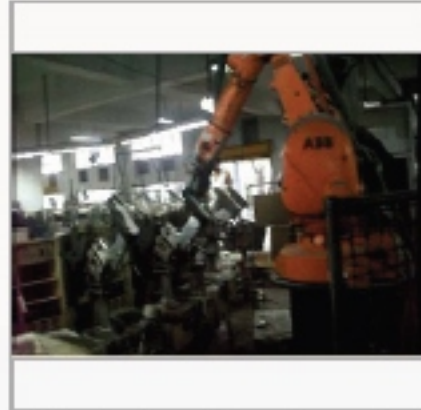
Robotic Roughing/Spraying
