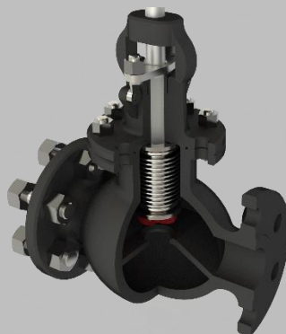
VALVE BELLOWS
