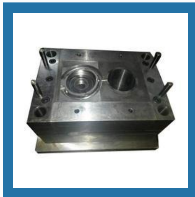
Steel Transfer Molding Dies
