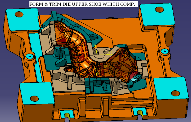
FORM & TRIM DIE UPPER SHOE WITH COMP.
