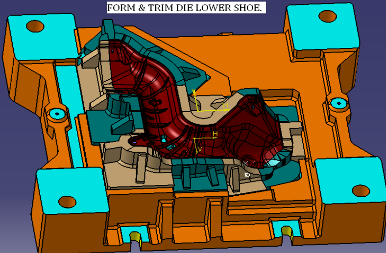
FORM & TRIM DIE LOWER SHOE.
