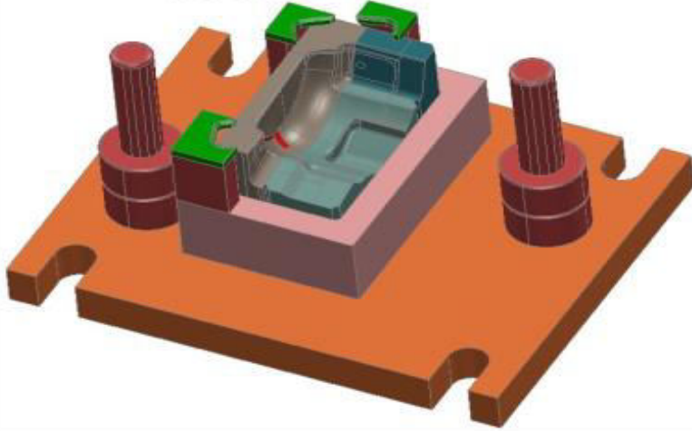
FORM DIE LOWER SHOE
