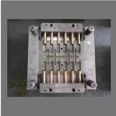
Inline Dripper Mould
