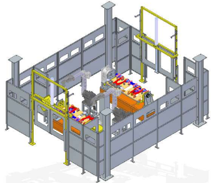
Robotic Welding
