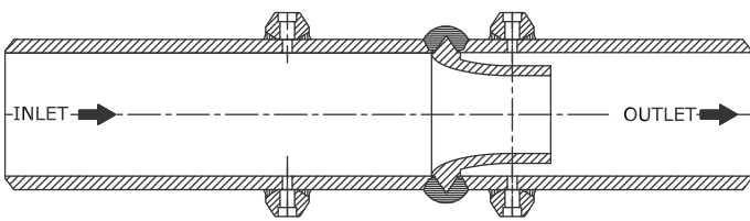
Long Radius High Beta, Weldin Type
